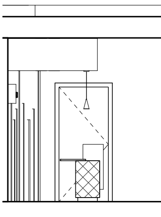
② Section View 1/4" = 1'-0"
